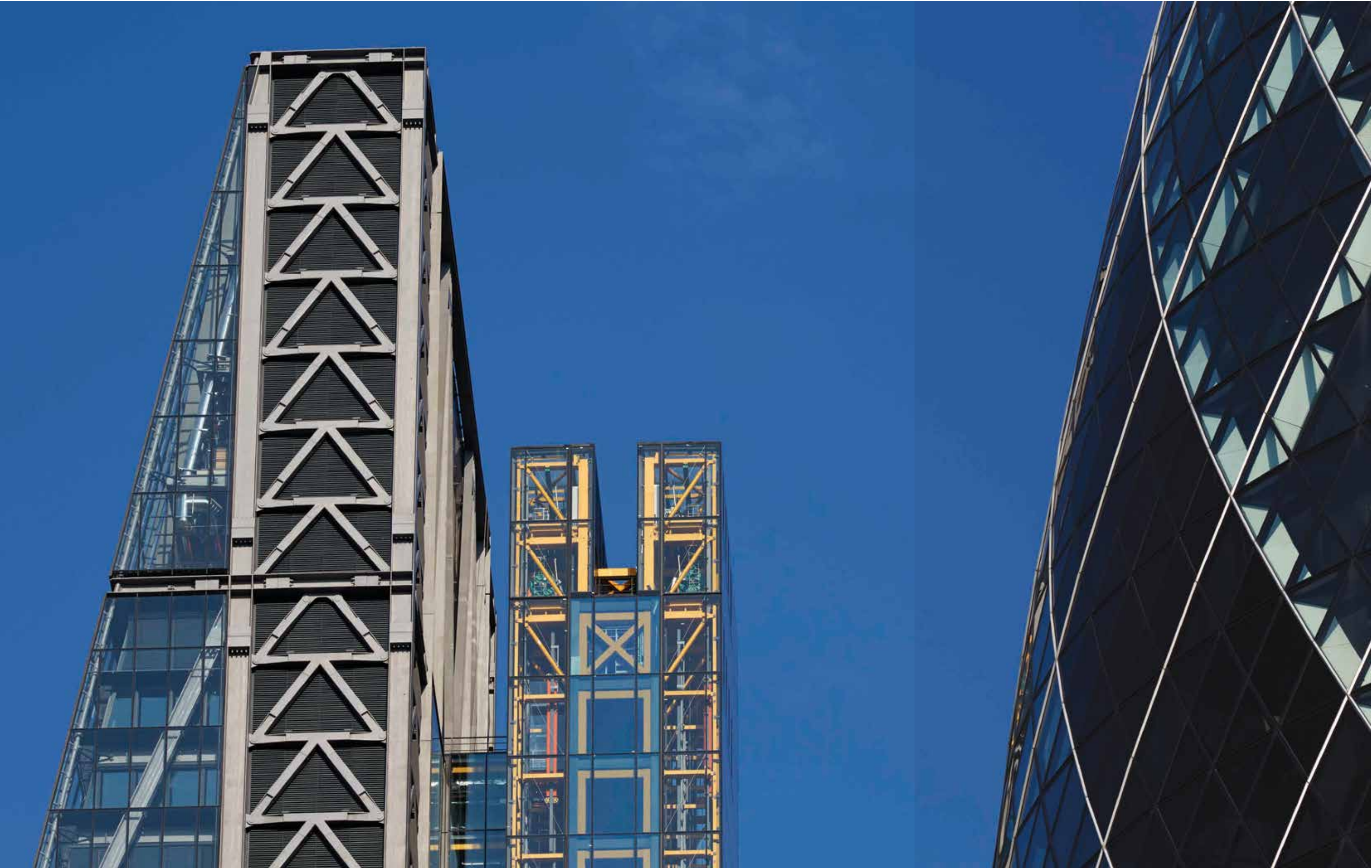
Detail of K-Bracing at the top ofThe Leadenhall Building | Richard Bryant, 2014 | Courtesy of British Land/Oxford Properties
